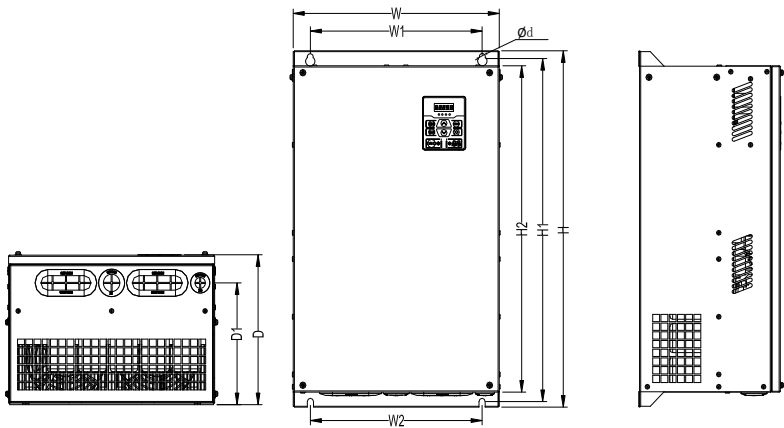
(b) A90-4T060~A90-4T304 变频器外形
