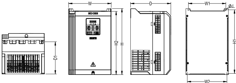
(a) A90-4T1R5B~A90-4T045B 变频器外形
